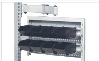
Rotating tool panel frame with M500 perforated panel, M500 bin rails and 8 plastic ESD bins
