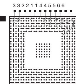
BGA352/388/420/456/480/516 Universal 1.27mm DC70/72/85/90
