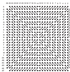
LBGA672T1.0-DC268
