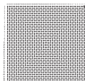
LBGA1936T1.0-DC449
