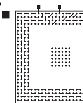
BGA352/388 DC70/72 1.27mm
