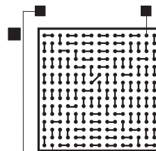
BGA225-DC15 1.5mm
