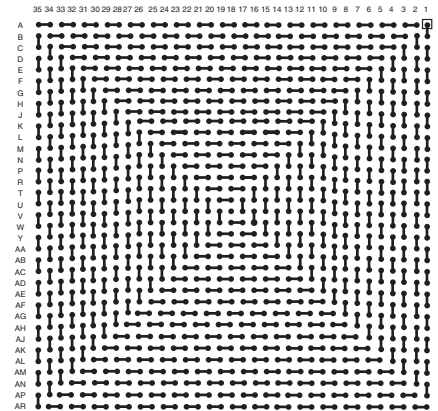
LBGA1225T1.27-DC359
