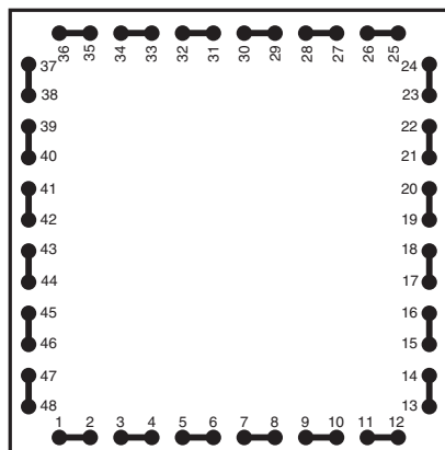
FC48 (PB18 - 250x250)
