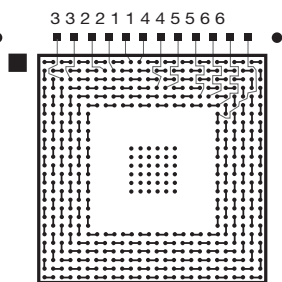
BGA352/388/420/456/480/516 Universal 1.27mm DC70/72/85/90
