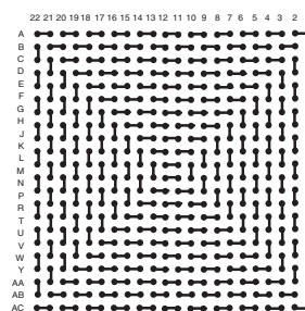
LBGA484T1.0-DC229A
