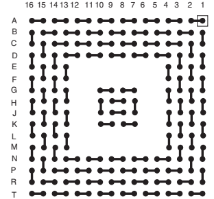
BGA208T1.0-DC164A
