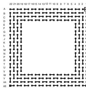
BGA288T1.0-DC221
