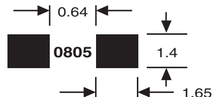
Pad Dimensions (mm) Rev-A
