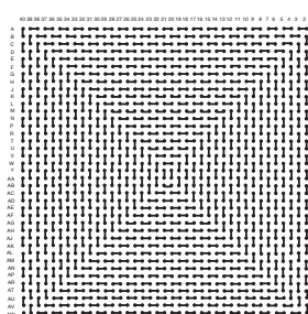
LBGA1600T1.0-DC409
