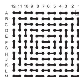
LBGA144T1.0-DC128
