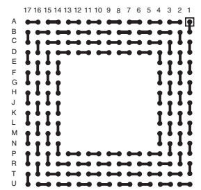
LBGA208T.8-DC170
