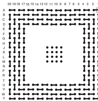
BGA272T1.27-DC202
