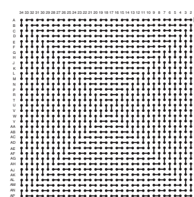
LBGA1156T1.0-DC349
