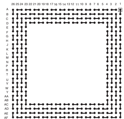
BGA352T1.27-DC70
