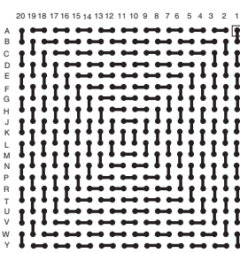
LBGA400T1.0-DC209
